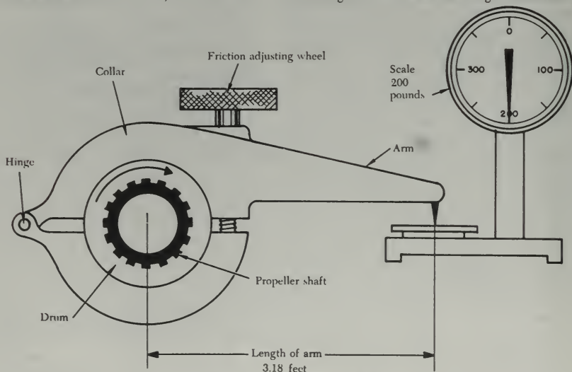
FIGURE 1-29. Typical Prony brake.
